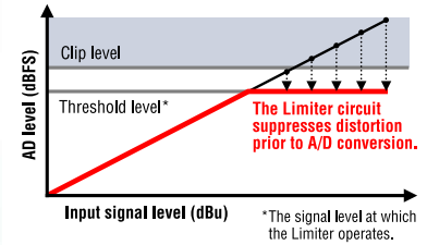
■ Limiter Operation
