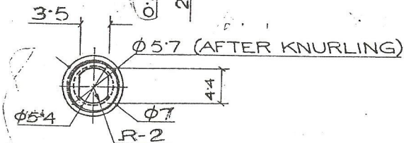
INSERT (2) MAT: BRASS
