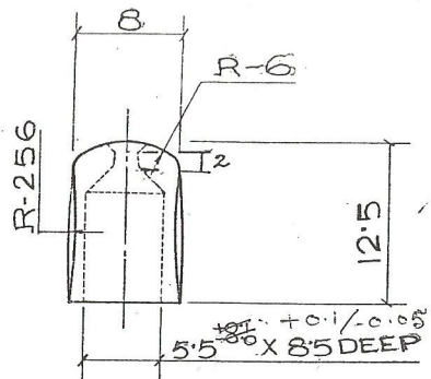
BUTTON HEAD (1) MAT: WOOD (EBONY).
